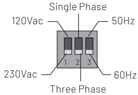
Figure 9: DIP Switches
